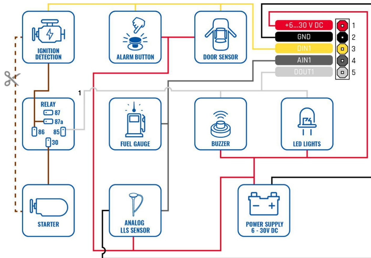
Figure 3 MTB100 Wiring scheme
