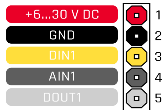
Figure 2 MTB100 pinout
